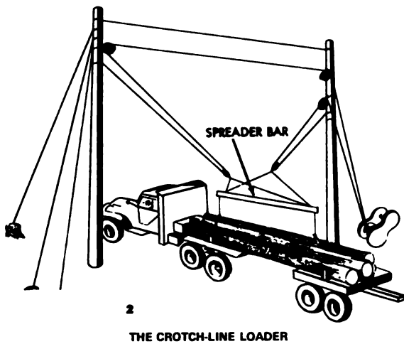
Figure 7-18. Loading devices.
